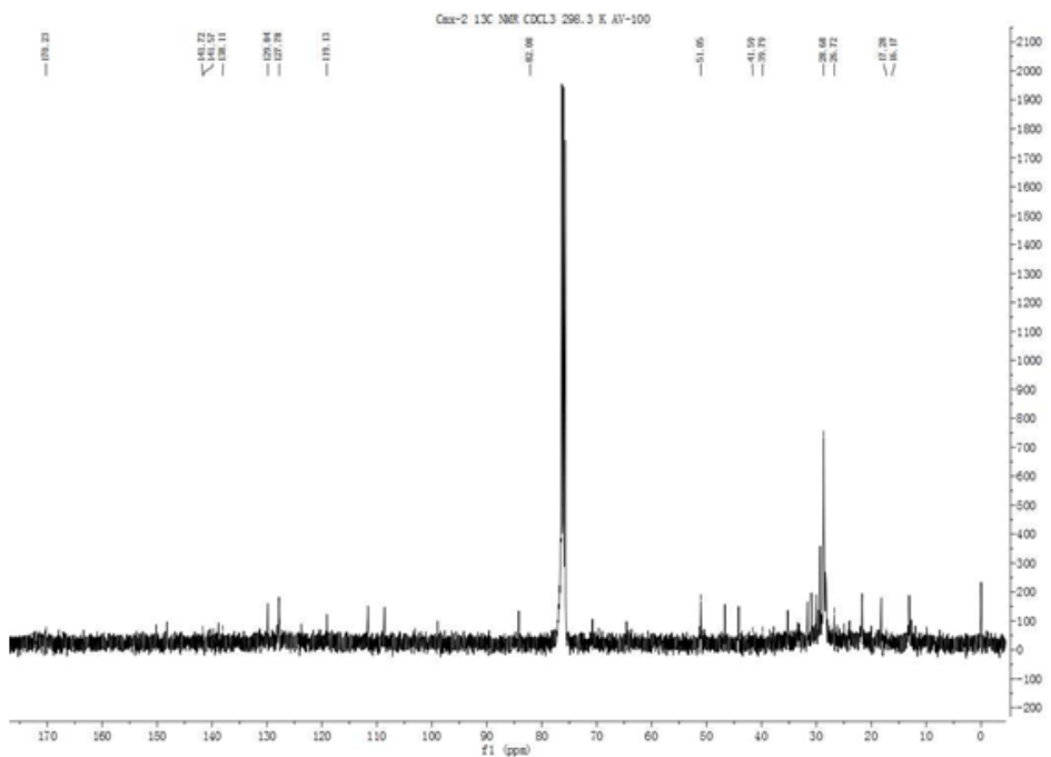
Supplementary Figure 4. The ^{13}\text{C} -NMR spectra of compound costunolide.
