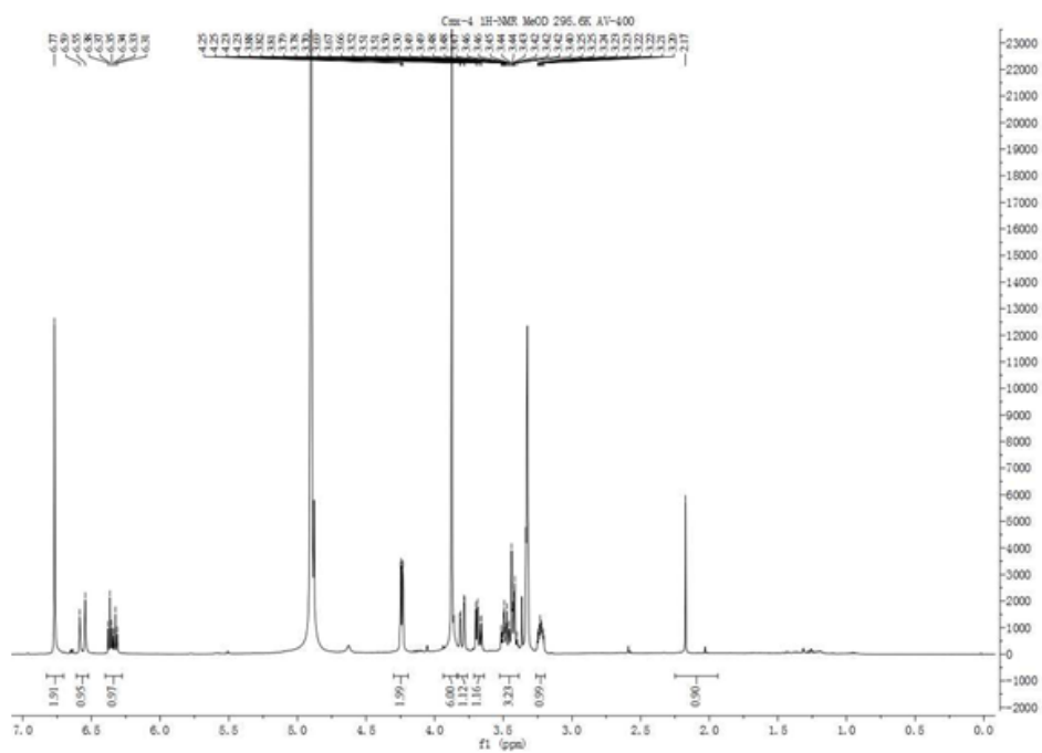
Supplementary Figure 1. The ^1\text{H} -NMR spectra of compound syringin.
